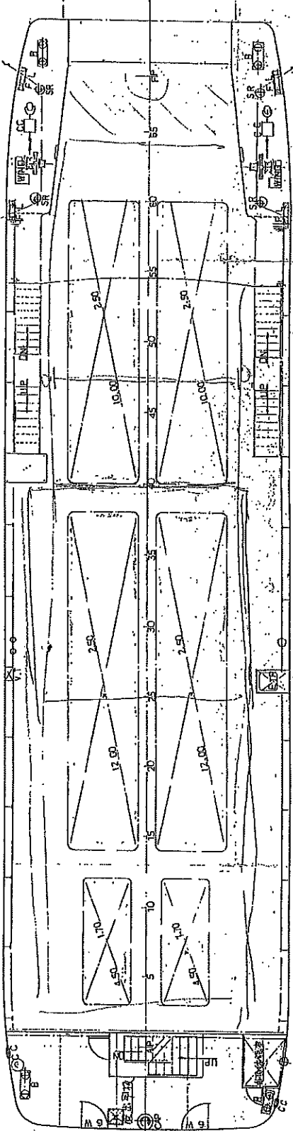
WAGON DECK PLAN
