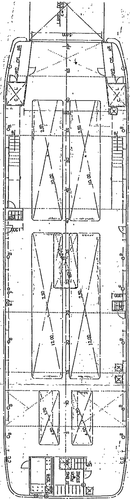
WAGON DECK PLAN
